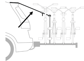
Tension-relief strap
